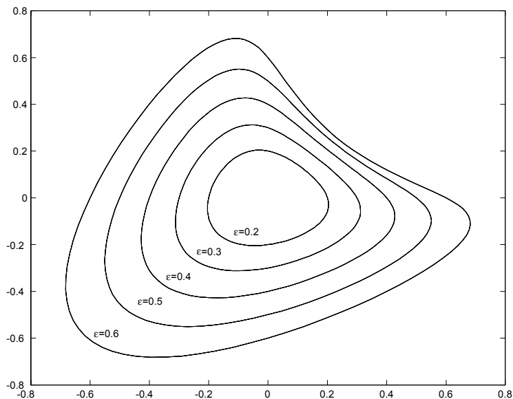
Figure 1: Image of the quadratic map
